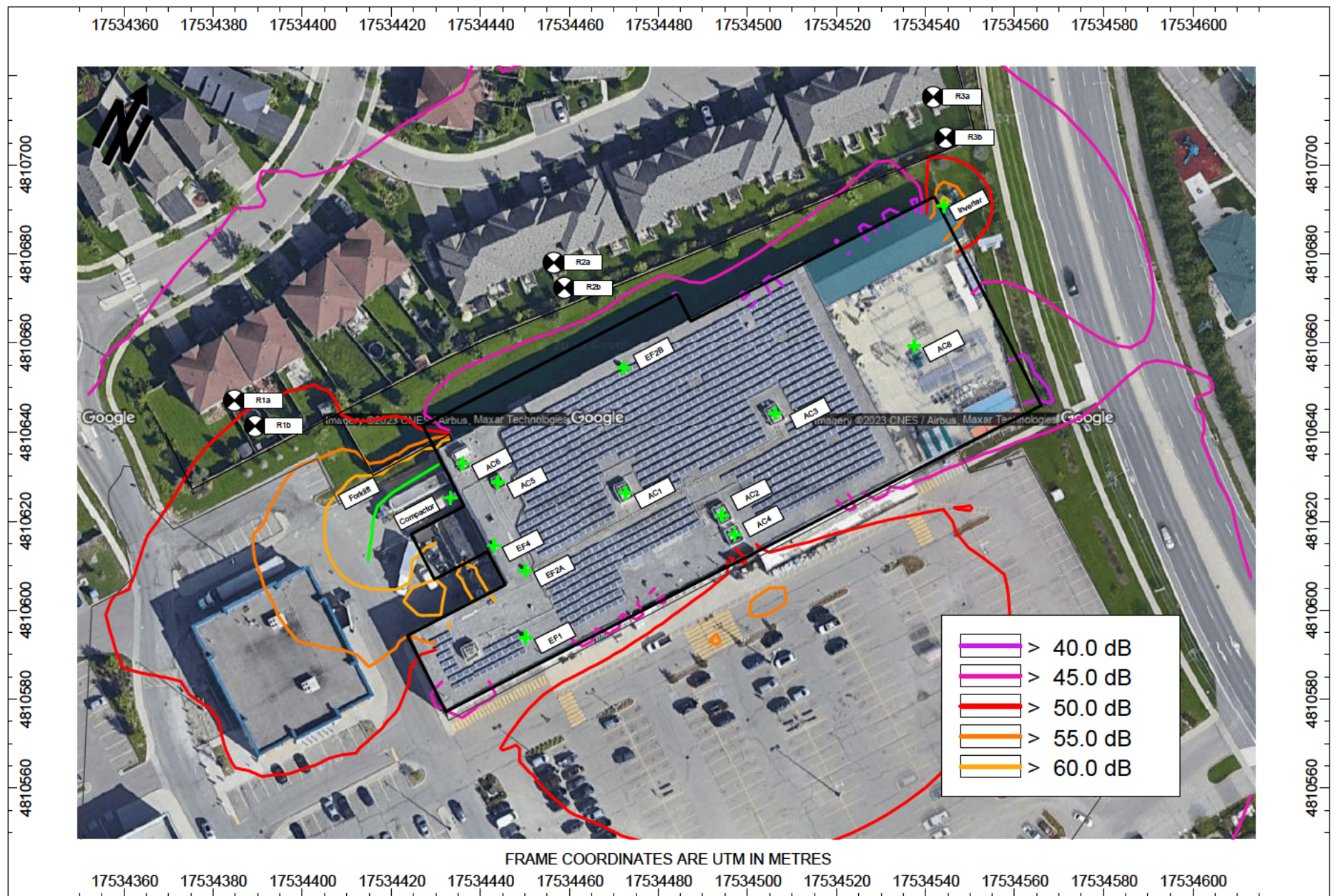
Figure 4a: Future Sound Level Contours, Leq [dBA] at 4.5 m Above Grade Daytime Hours (7:00 - 23:00)
