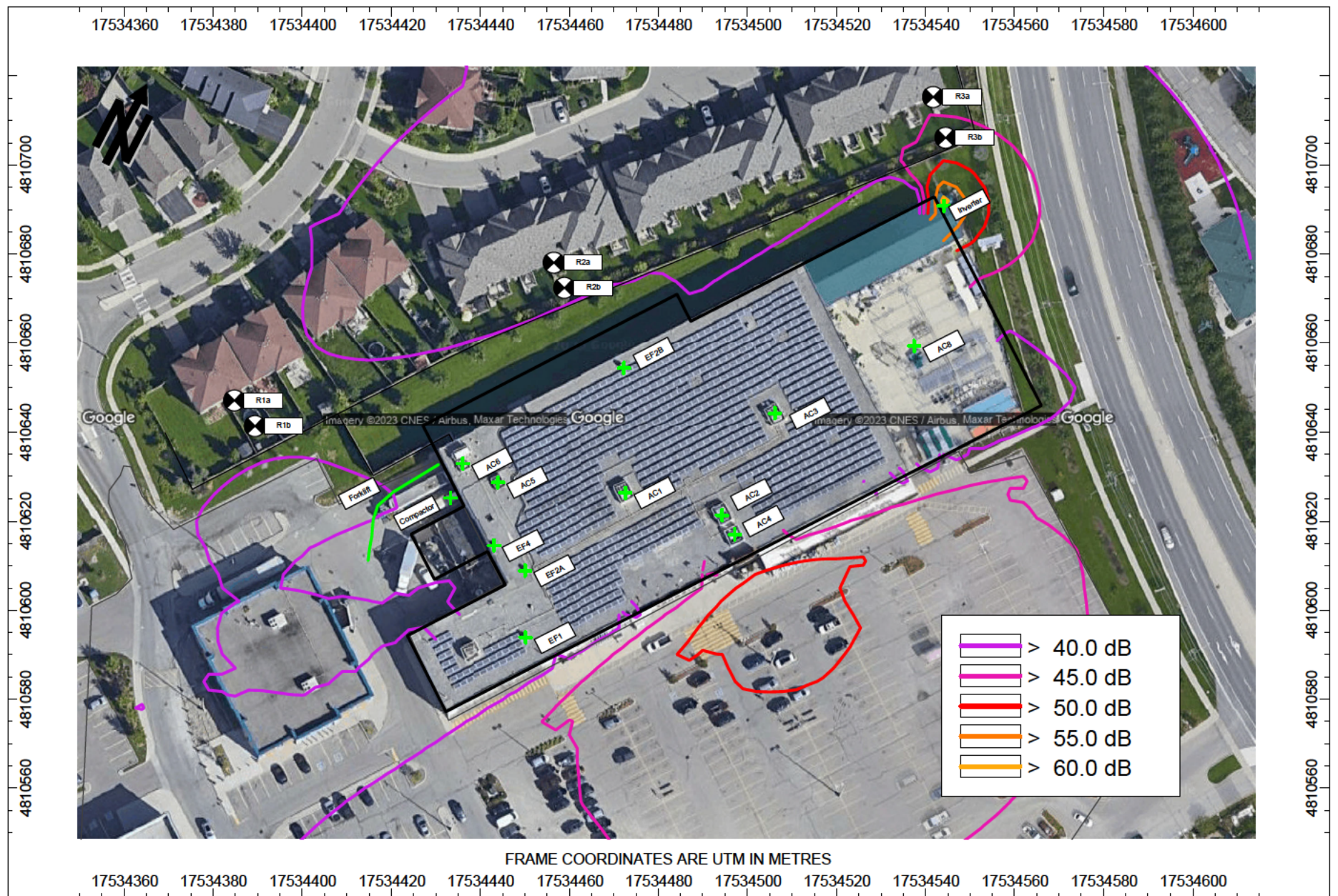
Figure 4b: Future Sound Level Contours, Leq [dBA] at 4.5 m Above Grade Night-time Hours (23:00 - 7:00)
