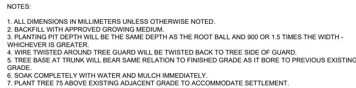
5 Coniferous Tree Planting On A Slope N.T.S.
