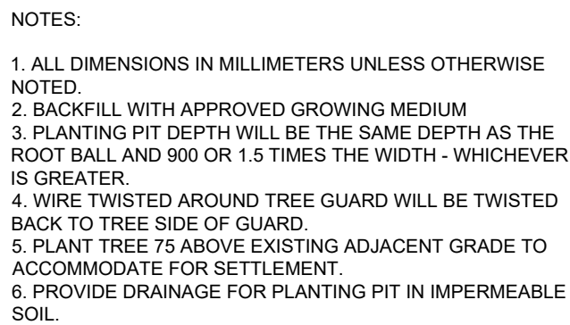
6 Deciduous Tree Planting On A Slope N.T.S.
